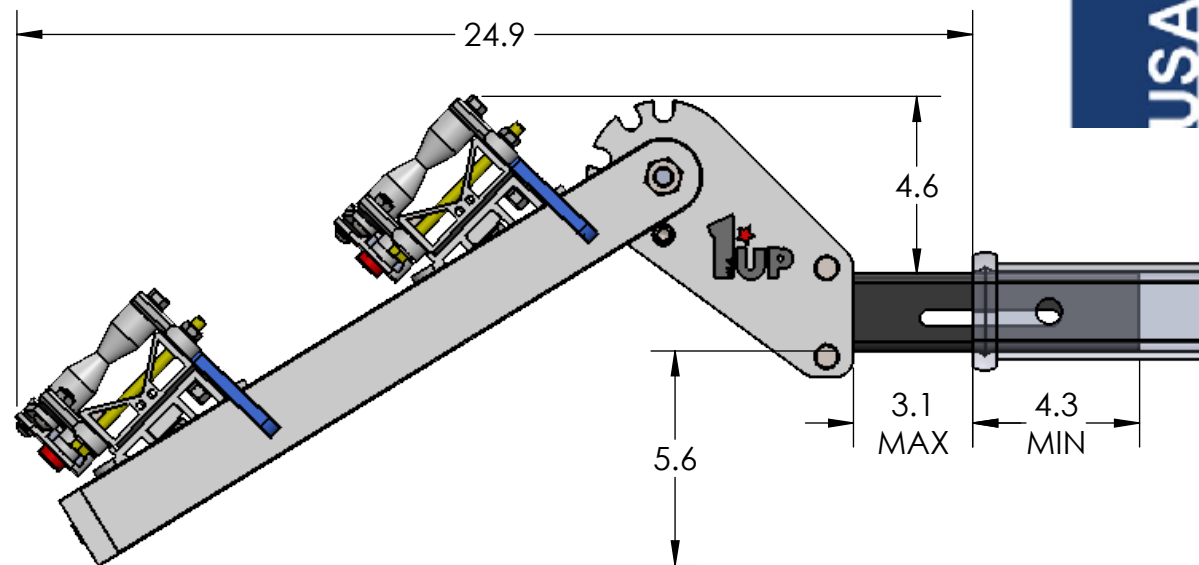
BASE RACK
